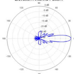
Elevation Antenna Pattern
